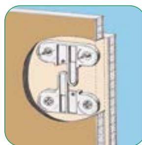
POLYTAC 2185 composed of two identical pieces for flat assembly.
