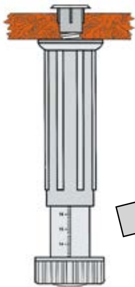
Furniture foot with dowel drilling ø 13 mm (dowel provided) Art. 4300 3 items available adjustable from 100 to 190 mm
