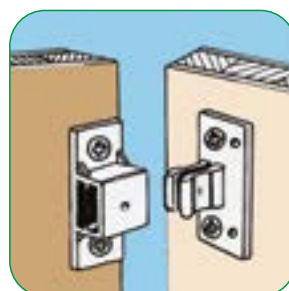
POLYTAC 2186 composed of two pieces (male/female) to clip together at 90°.
