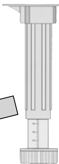
Furniture foot without advanced drilling Fastening with 4 screws(provided) Art. 4400 3 items available adjustable from 100 to 200 mm
